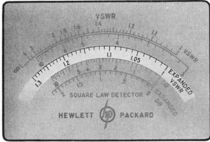
Fig. 2. Meter face used on new 415B SWI. 1-1.3 expanded VSWR scale shown accented. Expanded db scale is at bottom of meter face.
